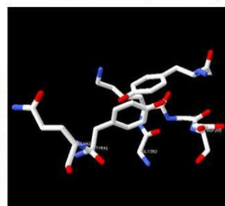
Y501 contacts (within 5Å)
