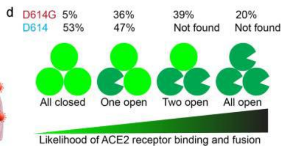
Fig 16: D614G Mutation Percentage
